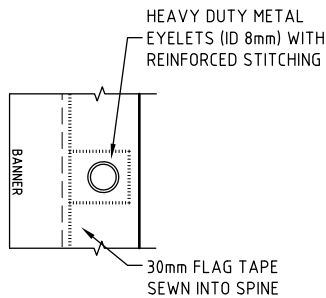
DETAIL 1 - OPTION 1 SCALE 1:2
