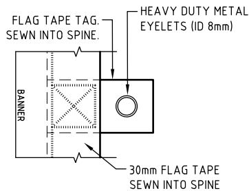
DETAIL 1 - OPTION 2 SCALE 1:2
